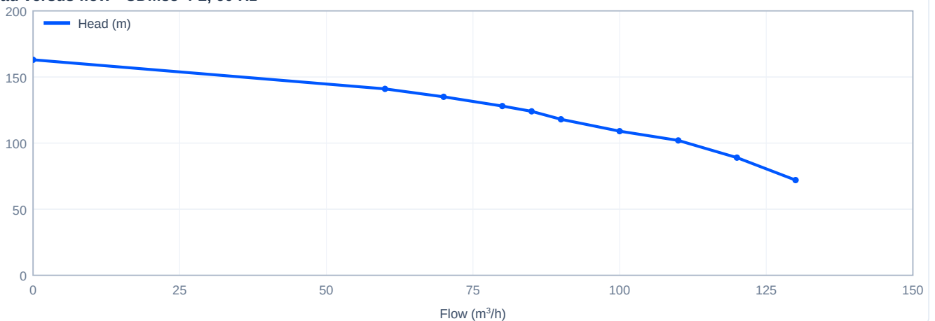
Head versus flow - CDM85-4-2, 60 Hz
