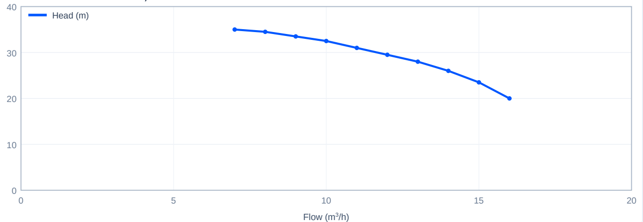
Head versus flow - CHL12-30G, 50 Hz
