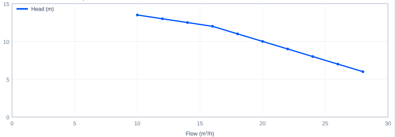
Head versus flow - CHL20-10, 50 Hz
