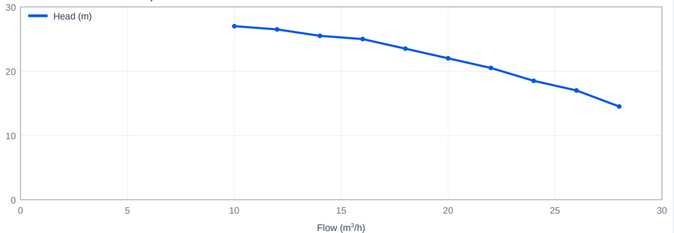
Head versus flow - CHL20-20G, 50 Hz
