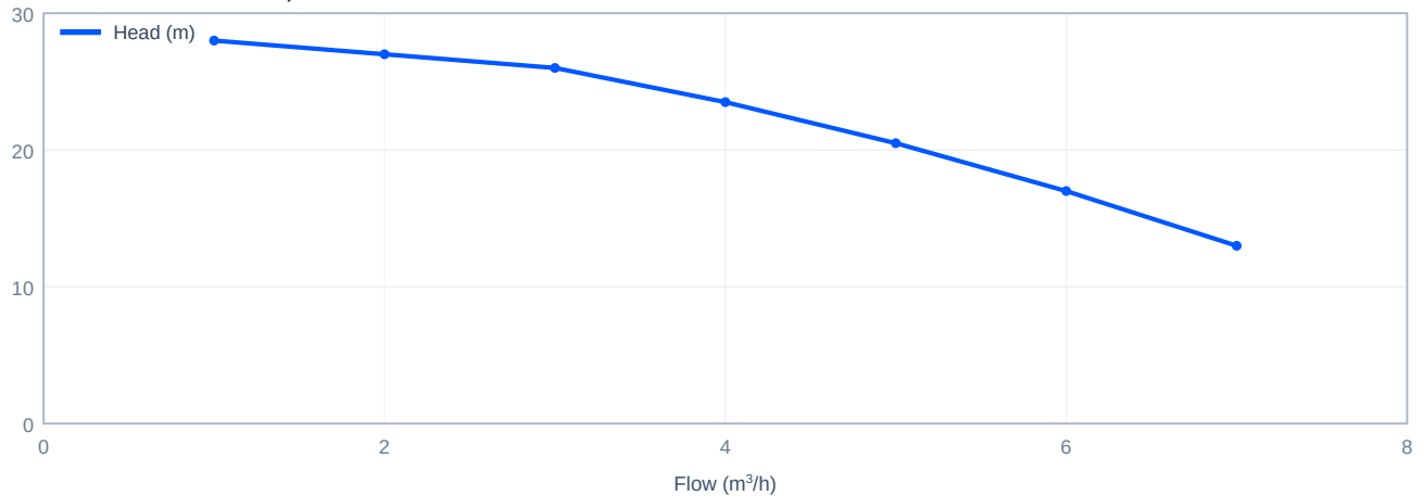
Head versus flow - CHL4-30, 50 Hz
