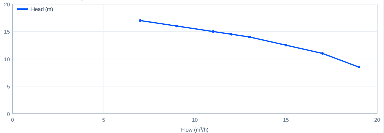
Head versus flow - CHL12-10, 60 Hz
