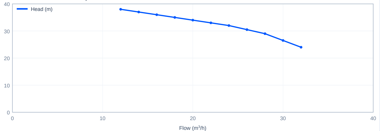
Head versus flow - CHL20-20G, 60 Hz
