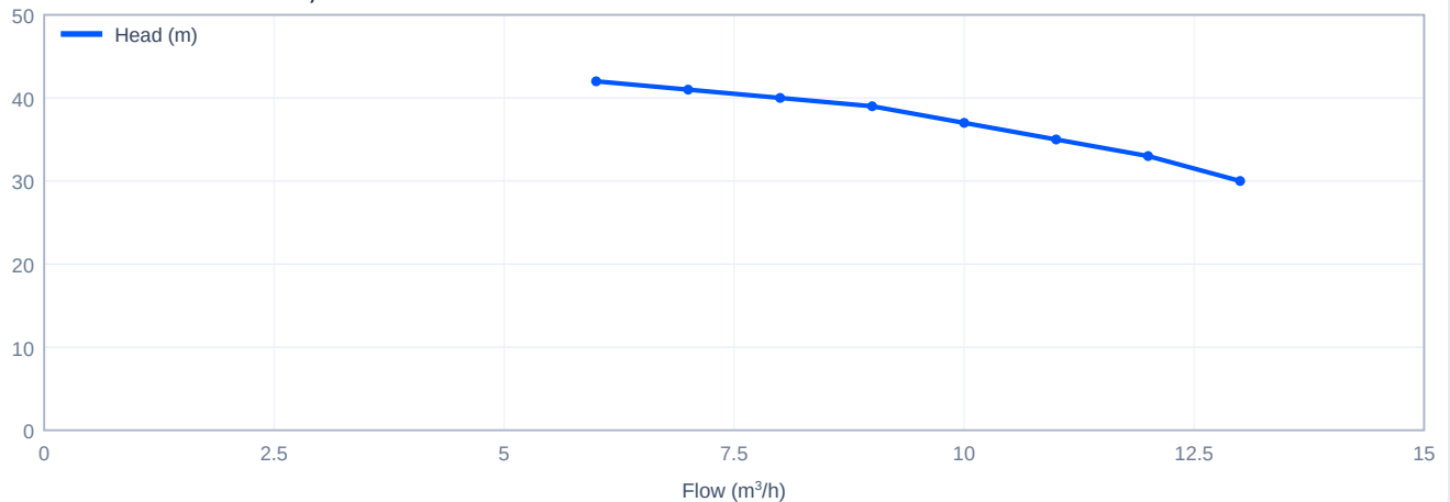
Head versus flow - CHL8-30G, 60 Hz
