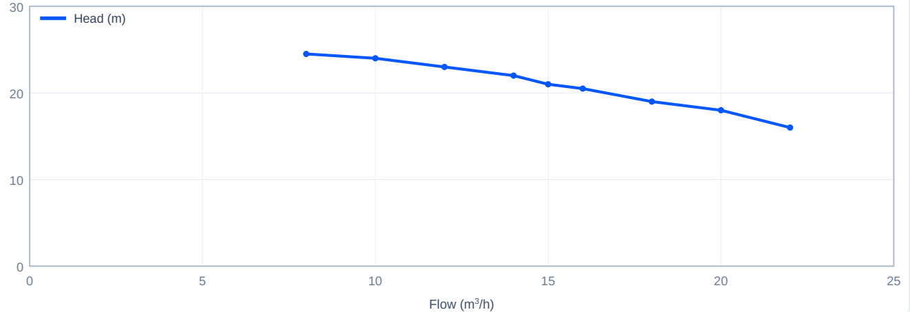
Head versus flow - CHLF(T)15-20, 50 Hz
