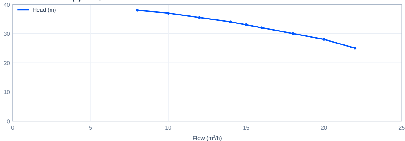
Head versus flow - CHLF(T)15-30, 50 Hz
