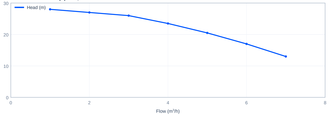
Head versus flow - CHLF(T)4-30, 50 Hz
