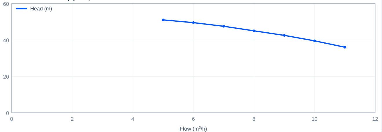
Head versus flow - CHLF(T)8-50, 50 Hz
