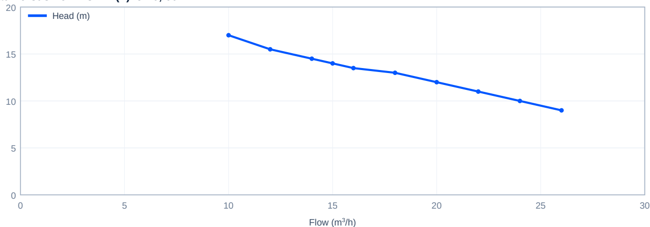
Head versus flow - CHLF(T)15-10, 60 Hz
