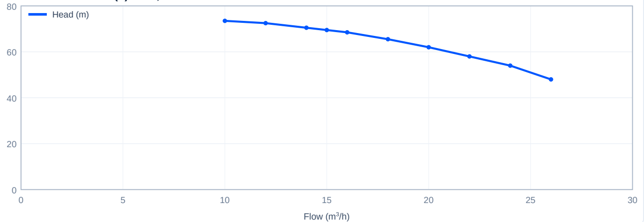
Head versus flow - CHLF(T)15-40, 60 Hz
