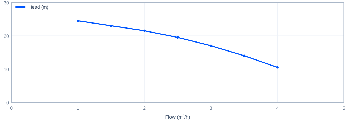
Head versus flow - CHLF(T)2-20, 60 Hz
