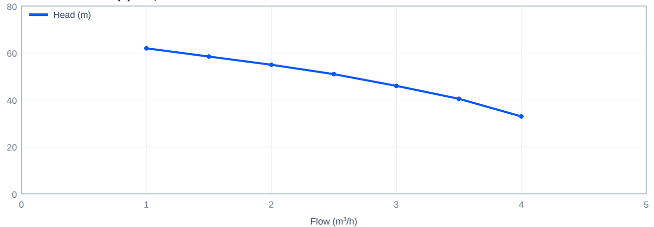
Head versus flow - CHLF(T)2-50, 60 Hz
