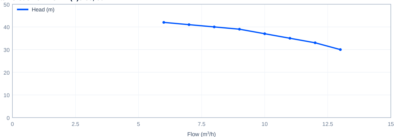
Head versus flow - CHLF(T)8-30, 60 Hz
