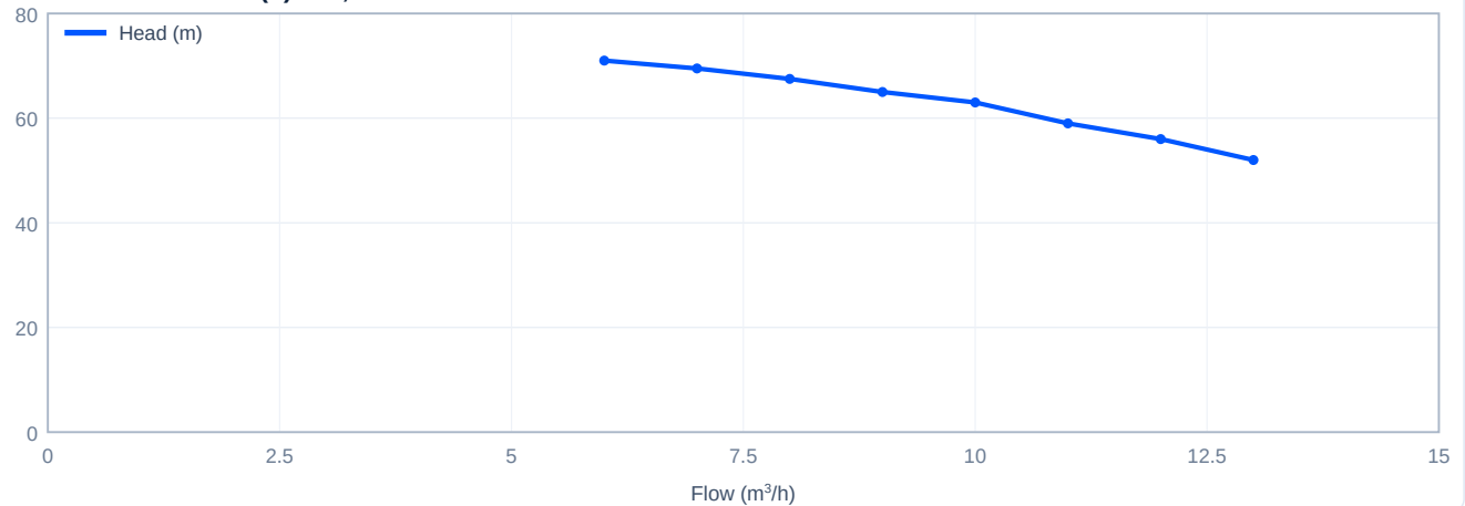
Head versus flow - CHLF(T)8-50, 60 Hz
