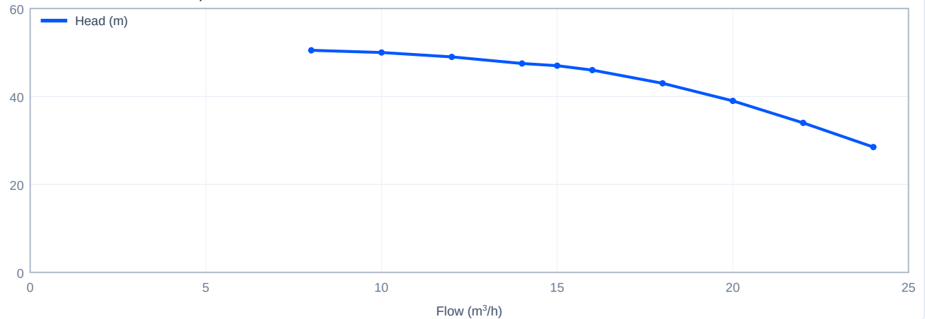
Head versus flow - CHM15-40, 50 Hz
