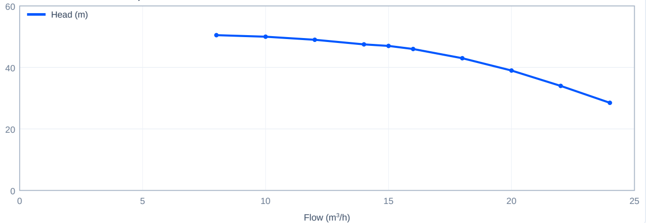
Head versus flow - CHM15-40, 50 Hz
