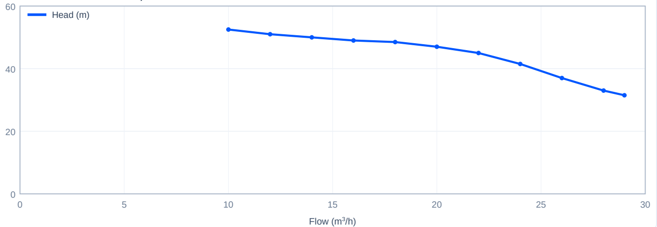
Head versus flow - CHM20-40, 50 Hz
