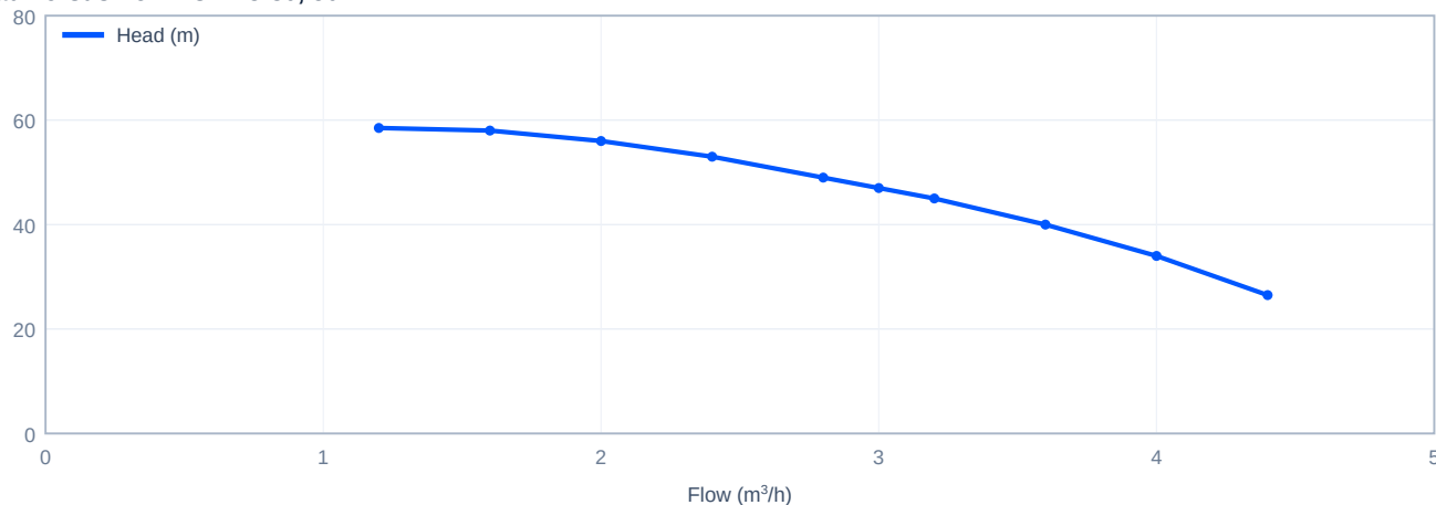
Head versus flow - CHM3-80, 50 Hz
