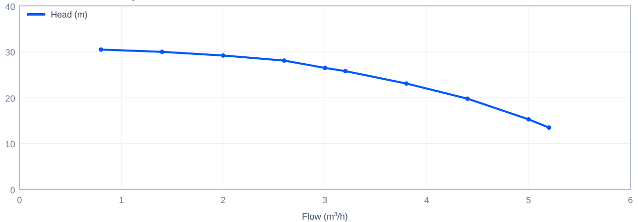
Head versus flow - CHME3-3, 50 Hz
