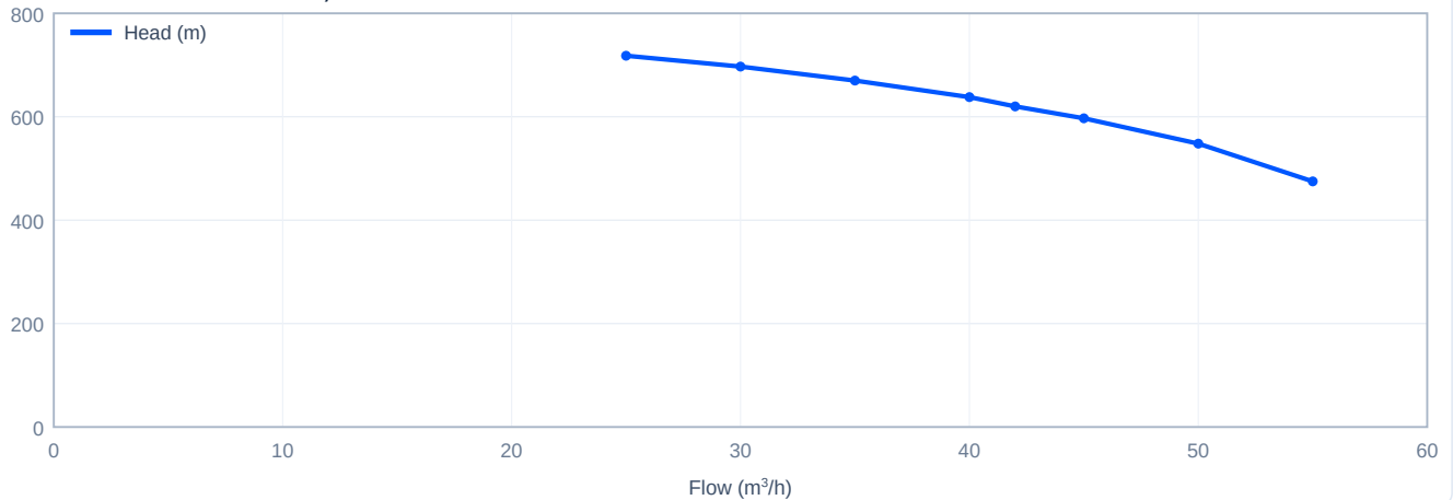
Head versus flow - HP42-15×2, 50 Hz
