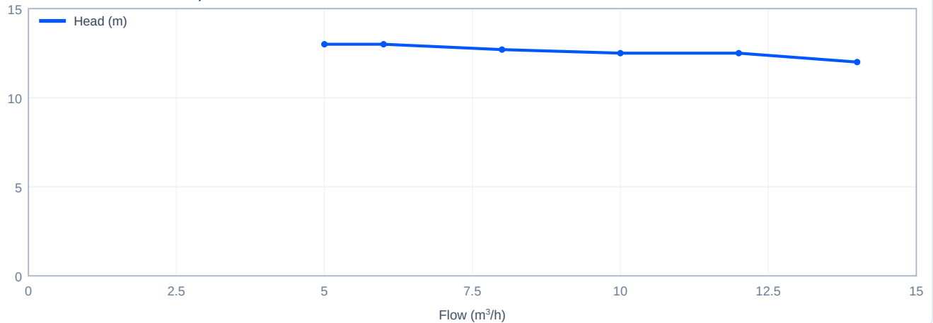
Head versus flow - LDMF10-1, 50 Hz
