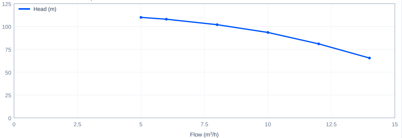
Head versus flow - LDMF10-10, 50 Hz
