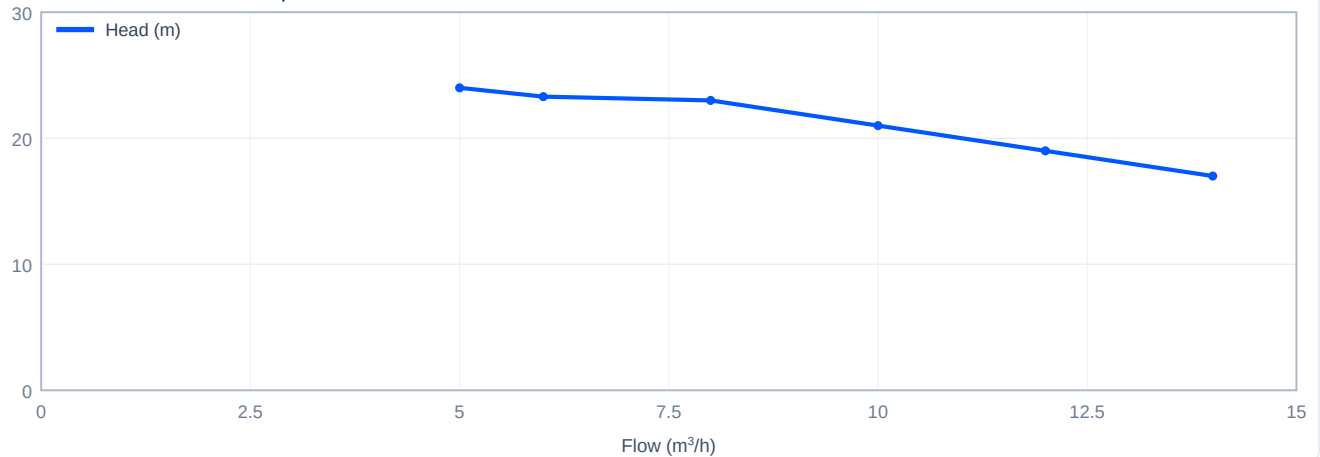
Head versus flow - LDMF10-2, 50 Hz
