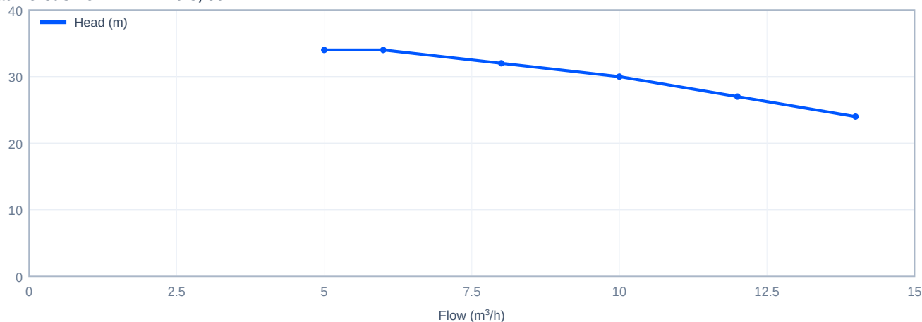
Head versus flow - LDMF10-3, 50 Hz
