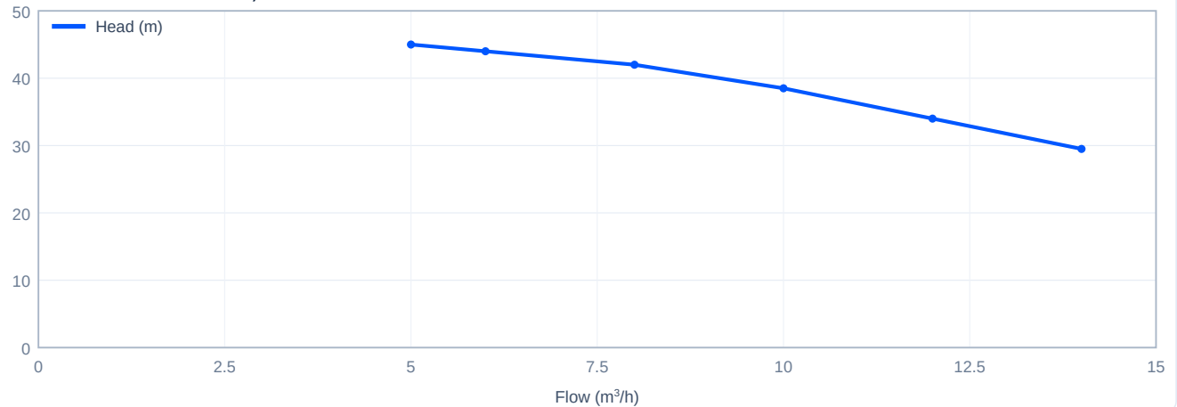
Head versus flow - LDMF10-4, 50 Hz
