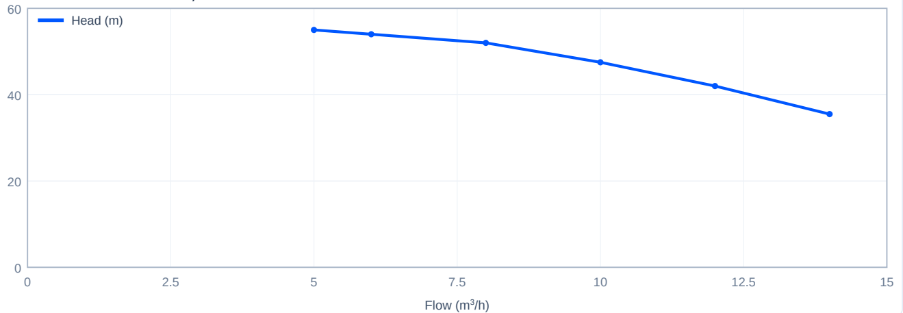
Head versus flow - LDMF10-5, 50 Hz
