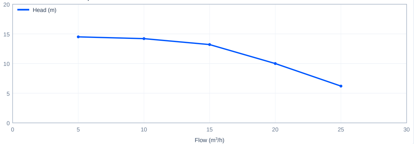
Head versus flow - NSA-L150, 60 Hz
