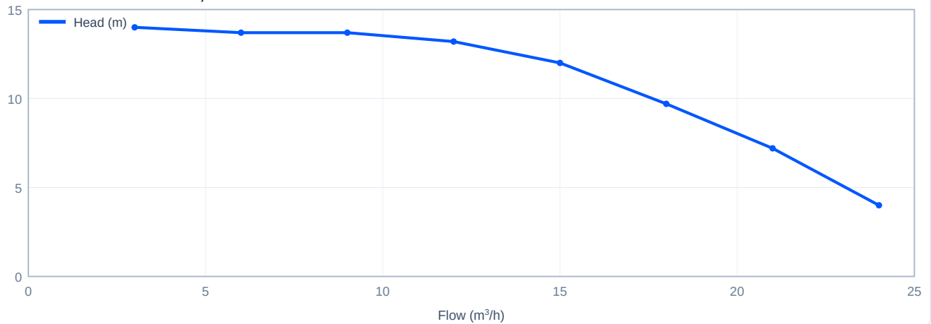
Head versus flow - NSW-L100, 60 Hz
