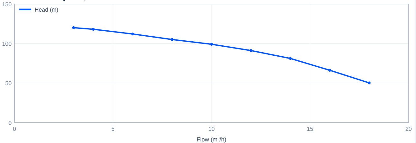
Head versus flow - PQ12-18, 50 Hz
