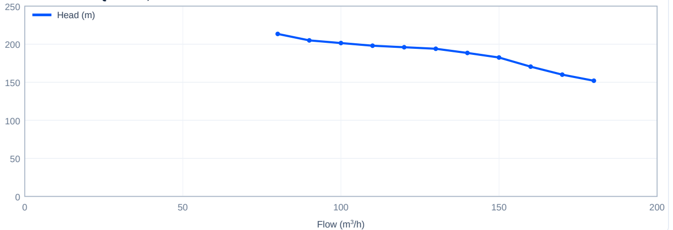
Head versus flow - PQ150-9-2, 50 Hz
