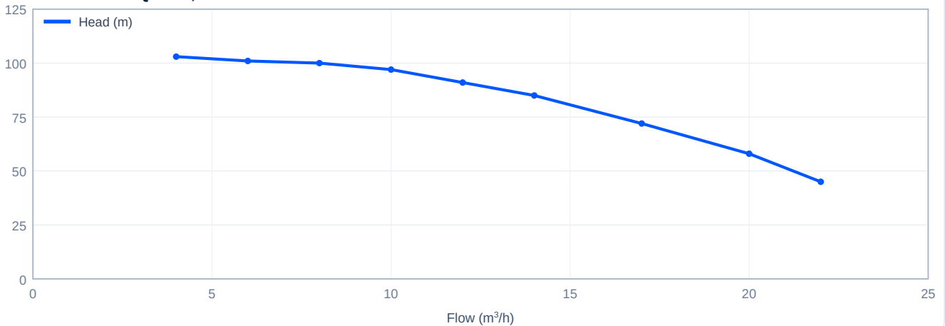
Head versus flow - PQ17-10, 50 Hz
