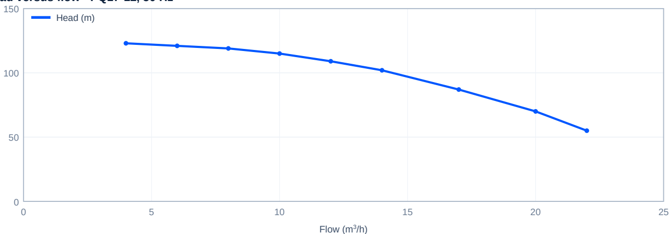
Head versus flow - PQ17-12, 50 Hz
