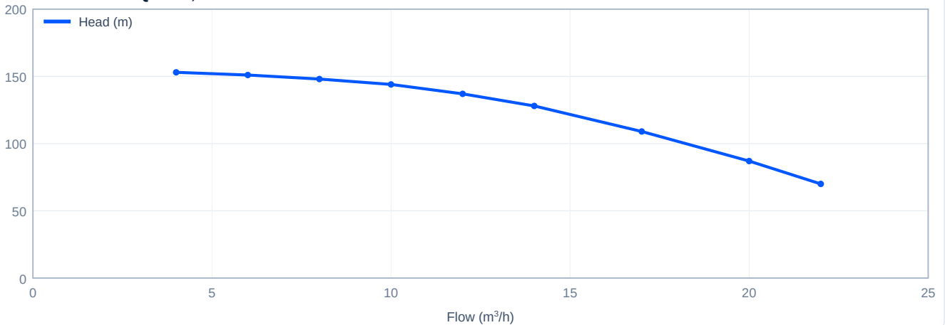
Head versus flow - PQ17-15, 50 Hz
