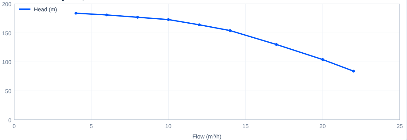
Head versus flow - PQ17-18, 50 Hz
