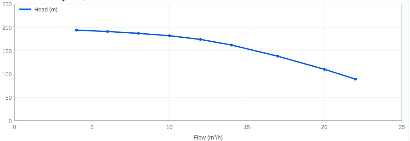
Head versus flow - PQ17-19, 50 Hz
