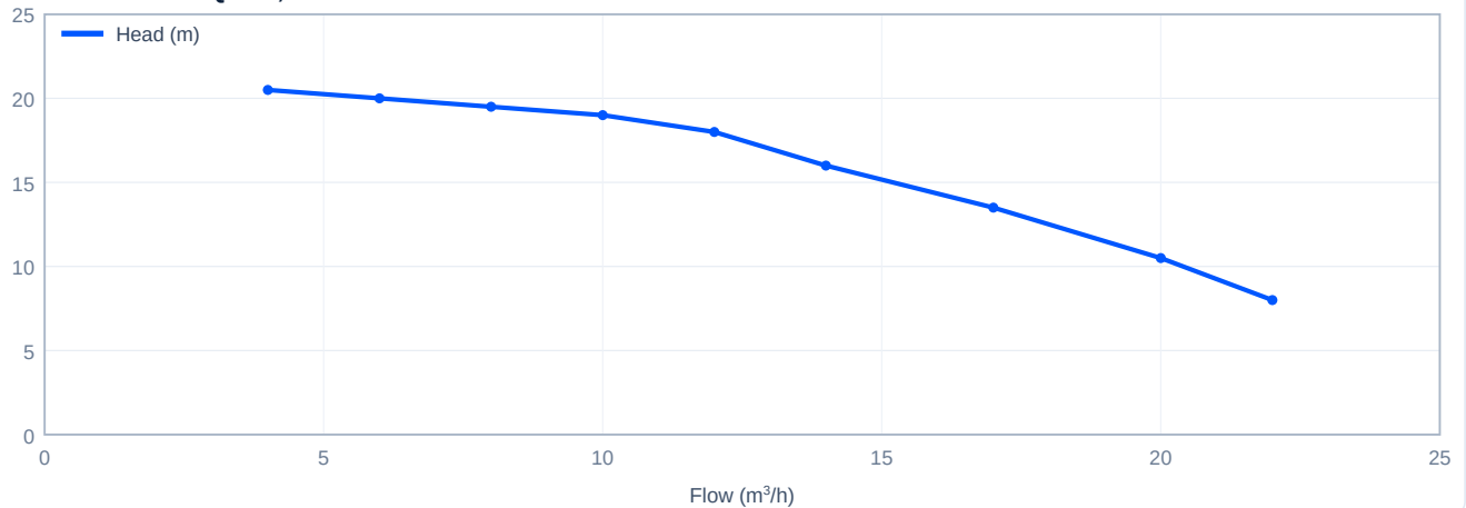
Head versus flow - PQ17-2, 50 Hz
