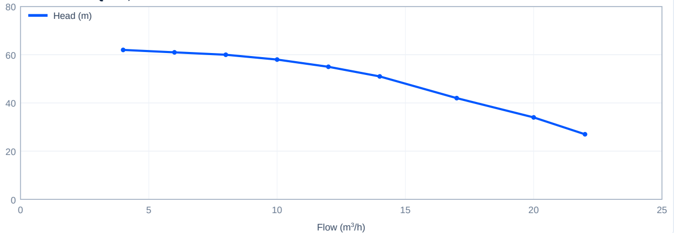
Head versus flow - PQ17-6, 50 Hz
