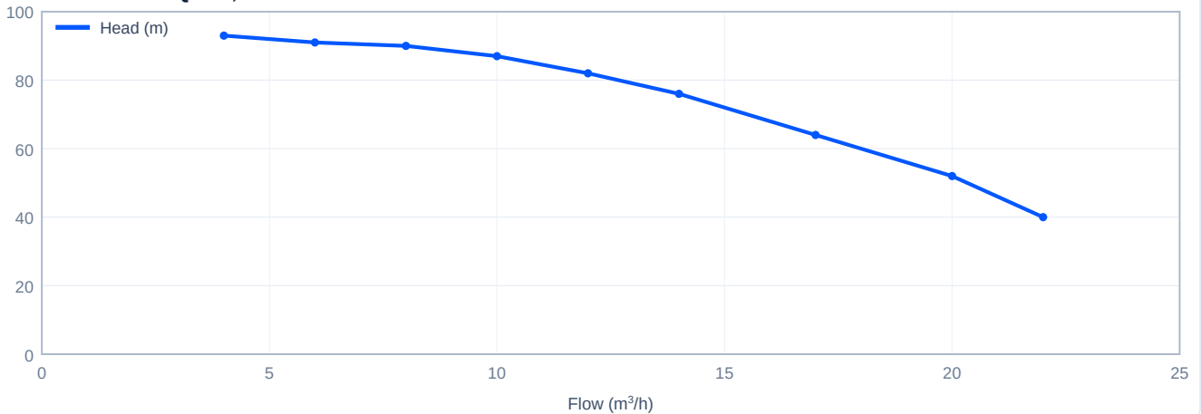
Head versus flow - PQ17-9, 50 Hz
