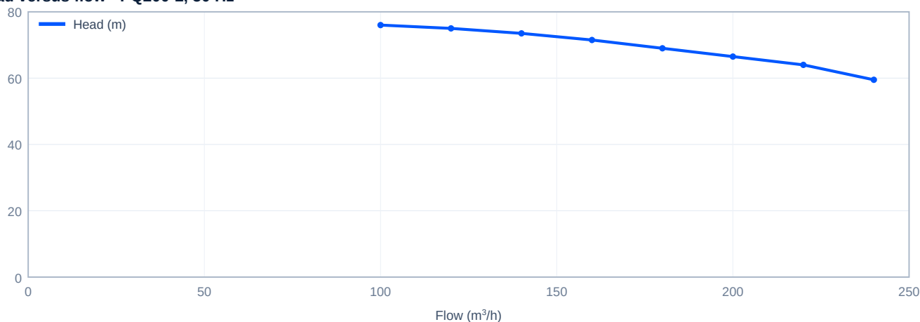
Head versus flow - PQ200-2, 50 Hz
