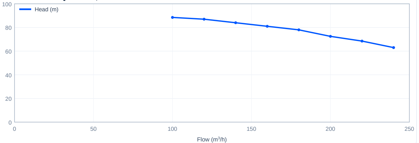
Head versus flow - PQ200-3-2B, 50 Hz
