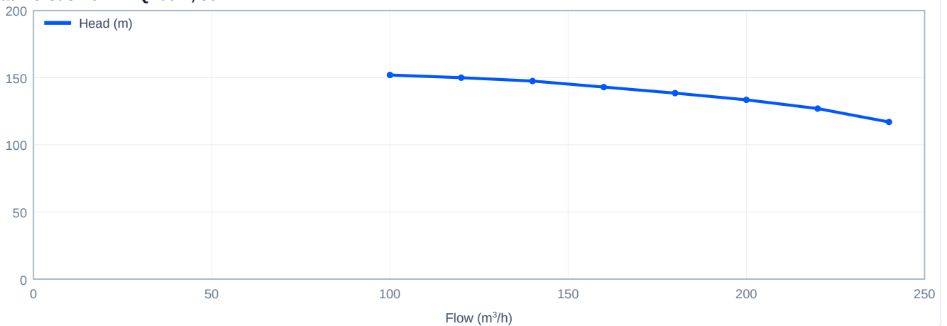
Head versus flow - PQ200-4, 50 Hz
