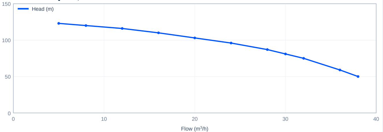
Head versus flow - PQ30-11, 50 Hz
