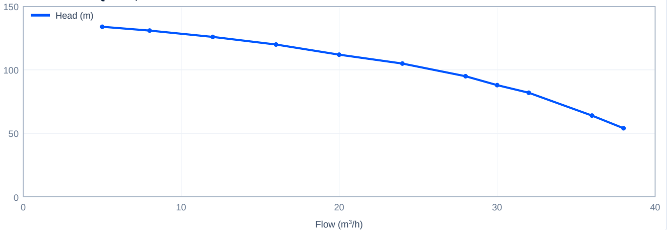
Head versus flow - PQ30-12, 50 Hz
