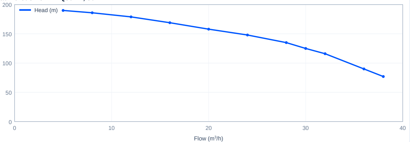
Head versus flow - PQ30-17, 50 Hz
