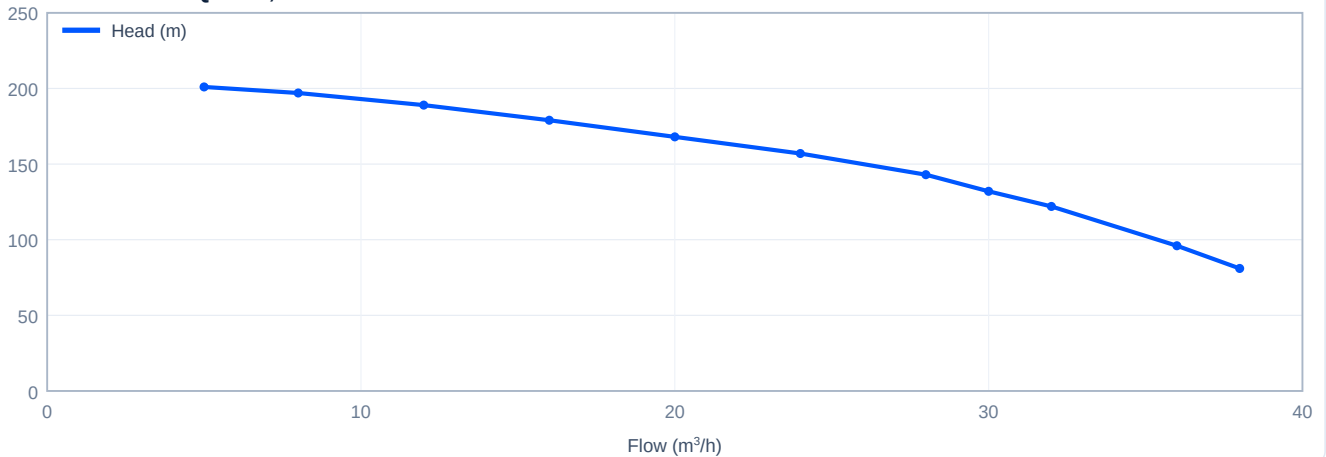
Head versus flow - PQ30-18, 50 Hz
