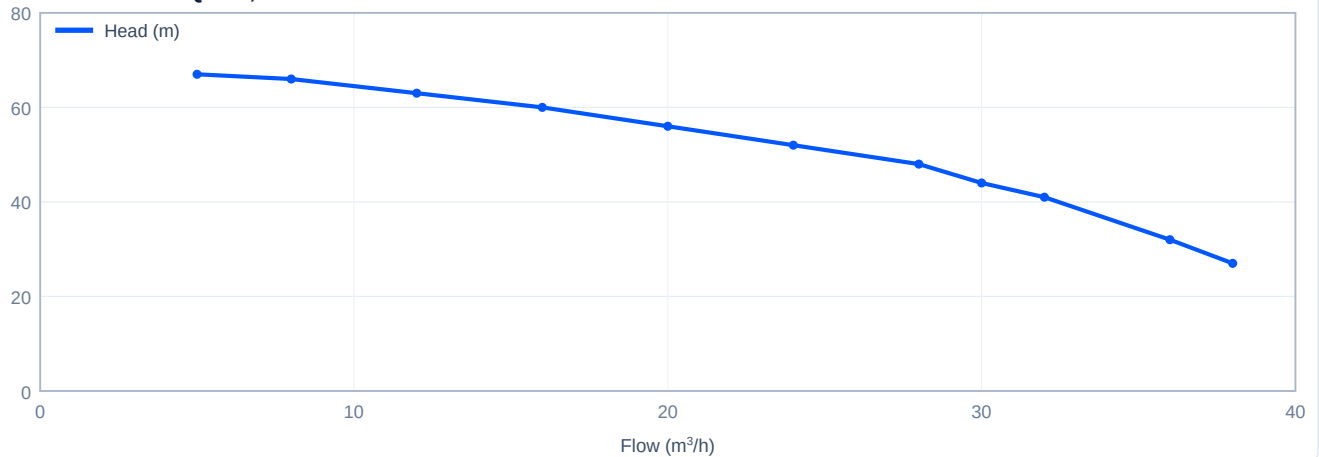
Head versus flow - PQ30-6, 50 Hz
