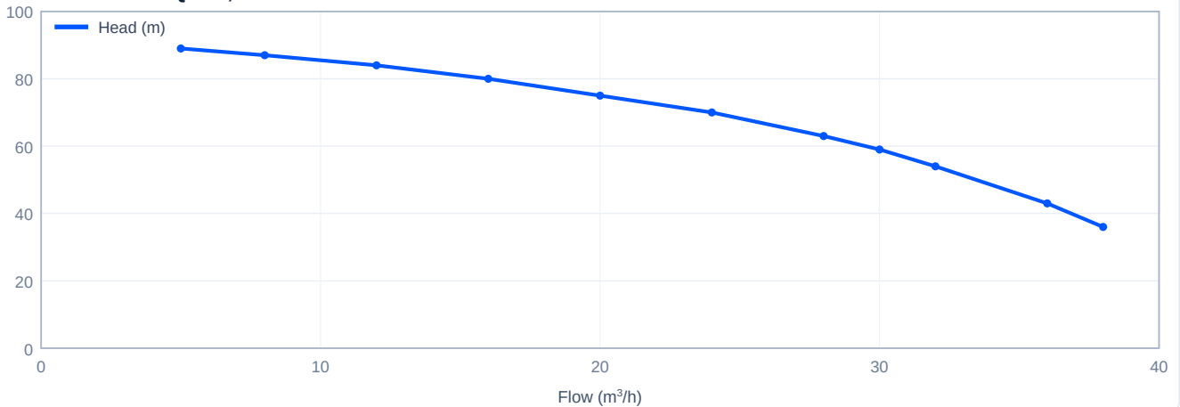
Head versus flow - PQ30-8, 50 Hz
